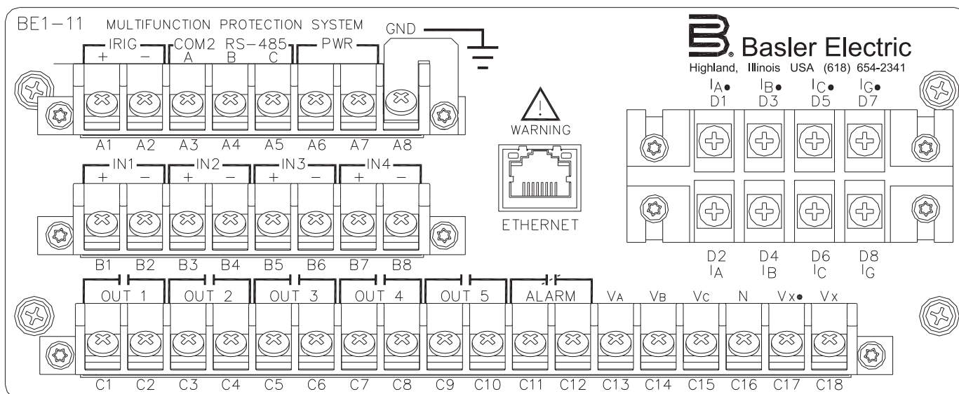
Figure 5 - BE1-11F H1 Rear Panel Connections (shown with optional Ethernet port)
