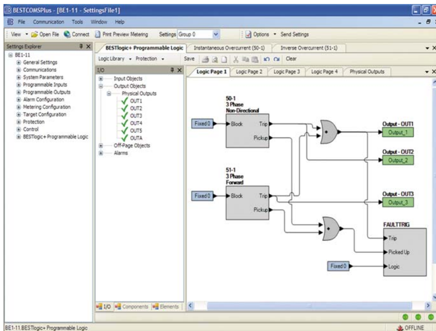
Figure 4 - BESTlogic+ Programmable Logic, Sample Screen
