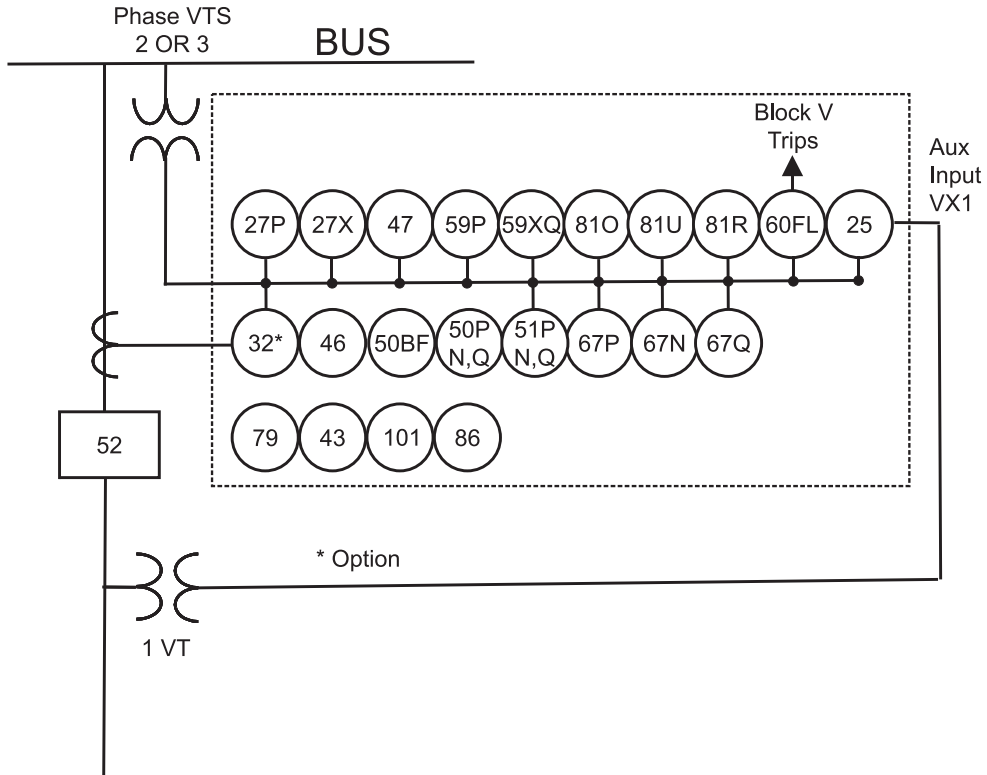
Figure 3 - BE1-11F Feeder Application
